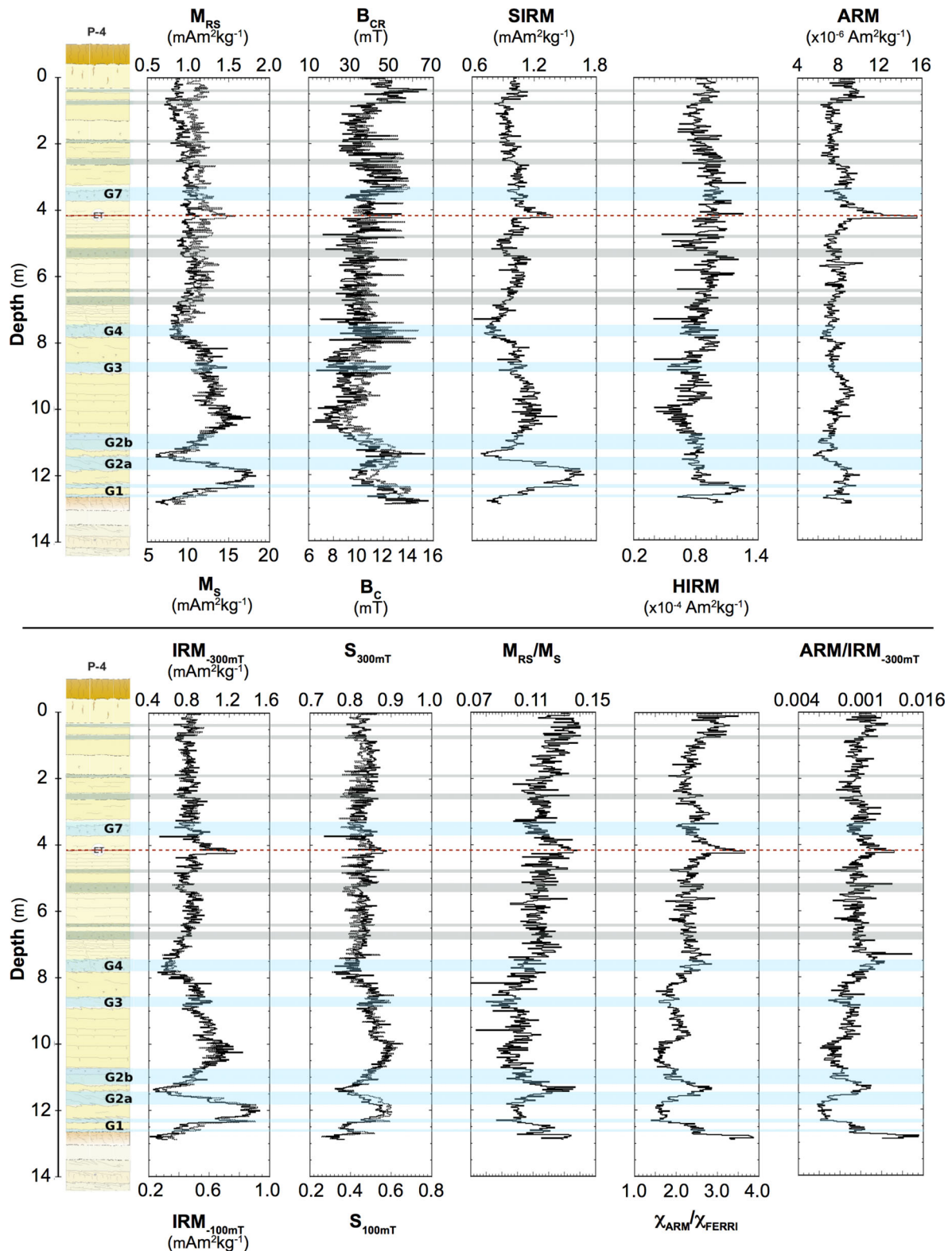
Figure 7. Variations of bulk magnetic parameters and ratios compared to the Nussloch P4 stratigraphy. M_{RS} , B_{CR} , IRM_{-300mT} and S_{300mT} are represented by the dashed lines in their respective plots. Grey and blue shaded horizons represent incipient and main tundra gley units, respectively. The Eltville Tuff (ET) tephra data at 4.22–4.20 m (red dotted line) are not shown.
