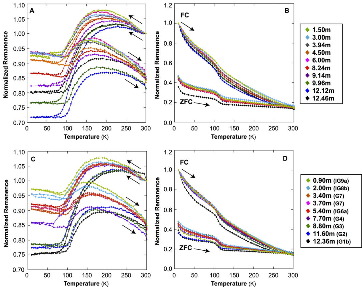
Figure 10. RT-SIRM (a, c) and ZFC/FC (b, d) data for a selection of samples within loess (upper panels) and tundra gley (lower panels) horizons. Note: G = main tundra gley; IG = incipient tundra gley. The arrows mark the cooling or warming direction for each curve.
