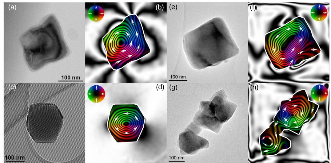
Figure 8. Electron holographic visualizations of single magnetic vortices in magnetite. (a) Bright-field TEM image of a particle ~250 nm in length. (b) Magnetic induction map reconstructed from electron holograms at room temperature (an in-plane saturating field was applied along the particle long axis to induce a remanent magnetization). (c and d) Electron hologram (with interference fringes used to calculate the magnetic contribution to the phase shift) and magnetic induction map for a hexagonal vortex state particle. Bright-field TEM image and induction map for a (e and f) single particle and (g and h) cluster of particles with nonvertically aligned vortex cores. All images are from the work of Almeida et al. (2016). The contour spacings (in radians) in the magnetic induction maps are 0.53 (Figure 8b), 0.78 (Figure 8d), 0.39 (Figure 8f), and 0.53 (Figure 8h); magnetization directions are indicated with arrows (depicted in the color wheels).
