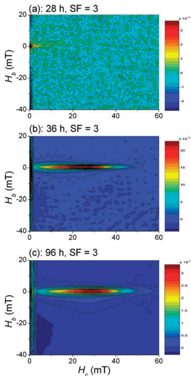
Figure 5. FORC diagrams for the AMB-1 cell sample at 28 (a), 36 (b) and 96 hr (c). A lower-left 'negative region' can be observed for the 96-hr sample.
