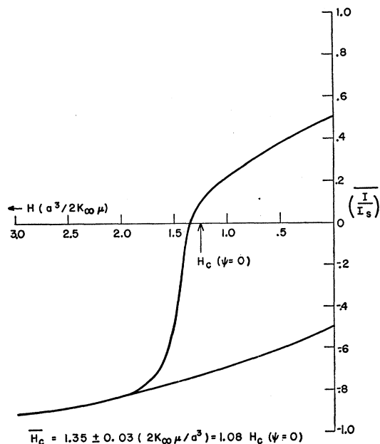
FIG. 6. Hysteresis loop of assembly of randomly oriented \infty -sphere chains (symmetric fanning mechanism).
