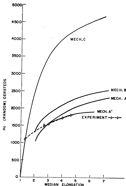
FIG. 8. Comparison of observed and calculated values of random coercive force of fine particle iron as a function of median elongation. Chain-of-spheres model: A —symmetric fanning mechanism; A' —nonsymmetric-fanning mechanism; B —parallel-rotation mechanism. Prolate spheroid model: C —parallel-rotation mechanism.
