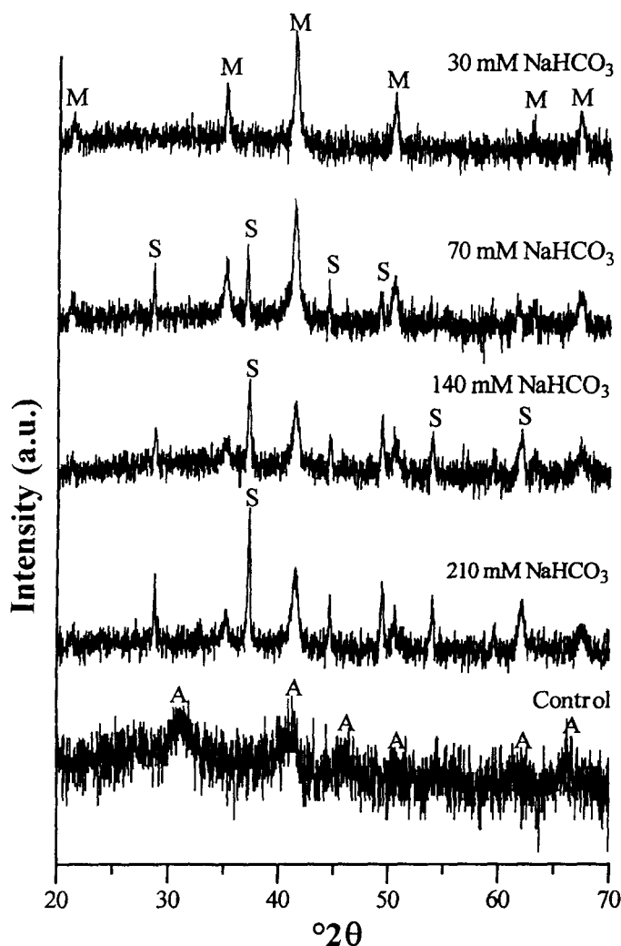
Figure 5. XRD patterns of Fe minerals formed by the Shewanella (NV-1) with different bicarbonate buffer concentrations under a N_2 atmosphere. A: akaganeite; M: magnetite; S: siderite.
