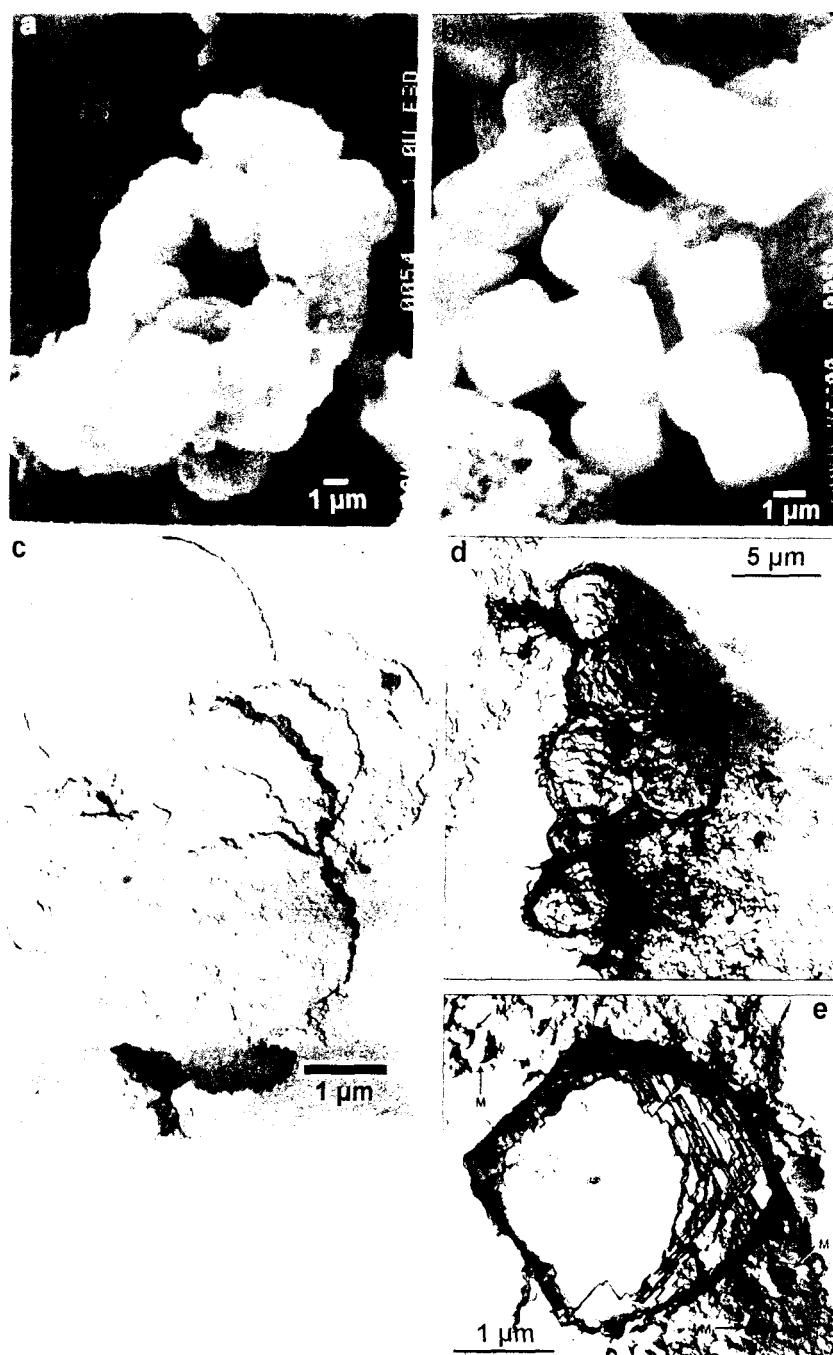
Figure 7. SEM images of magnetite and siderite formed by Shewanella and Thermoanaerobacter : (a) siderite globule formed by Shewanella (W3-7-1) under a H_2 - CO_2 atmosphere and (b) rhombohedral siderite formed by Shewanella (NV-1) under a H_2 - CO_2 atmosphere. TEM replica of siderite formed by Shewanella (BrY) and thermophilic Fe-reducing bacteria: (c) disk-like siderite formed by Shewanella (BrY), (d) siderite globule formed by the Thermoanaerobacter (TOR-39) using a medium buffered 90 mM NaHCO_3 , and (e) siderite coexisting with magnetite formed by the Thermoanaerobacter (TOR-39).
