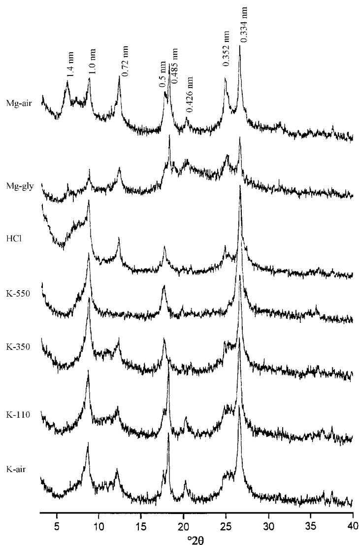
Figure 5. XRD patterns of the clay fraction in the C horizon of the pedon 901.
