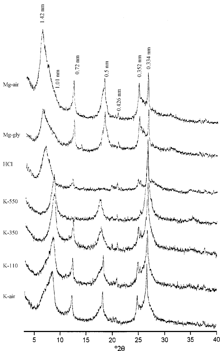
Figure 3. XRD patterns of the clay fraction in the Bh horizon of the pedon 901.
