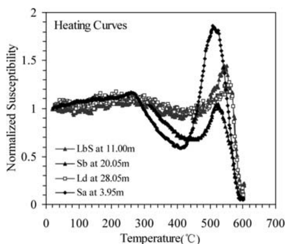
Figure 4. Heating curves of the loess, weakly developed palaeosol and palaeosol samples. For each sample, the susceptibility has been normalized by its room temperature susceptibility.
