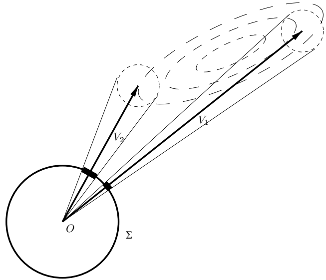
Figure A1. Applying the same 3-D Gaussian error \mathbf{g}_e(\mathbf{x}) (as symbolized by the two small-dash circles) to two different realizations \mathbf{V}_1 and \mathbf{V}_2 of a general 3-D Gaussian distribution \mathbf{g}(\mathbf{x}) (symbolized by the dashed ellipses), leads to different angular Gaussian errors on the unit sphere \Sigma if |\mathbf{V}_1| is larger than |\mathbf{V}_2| (as symbolized by the thick arcs on \Sigma ).
