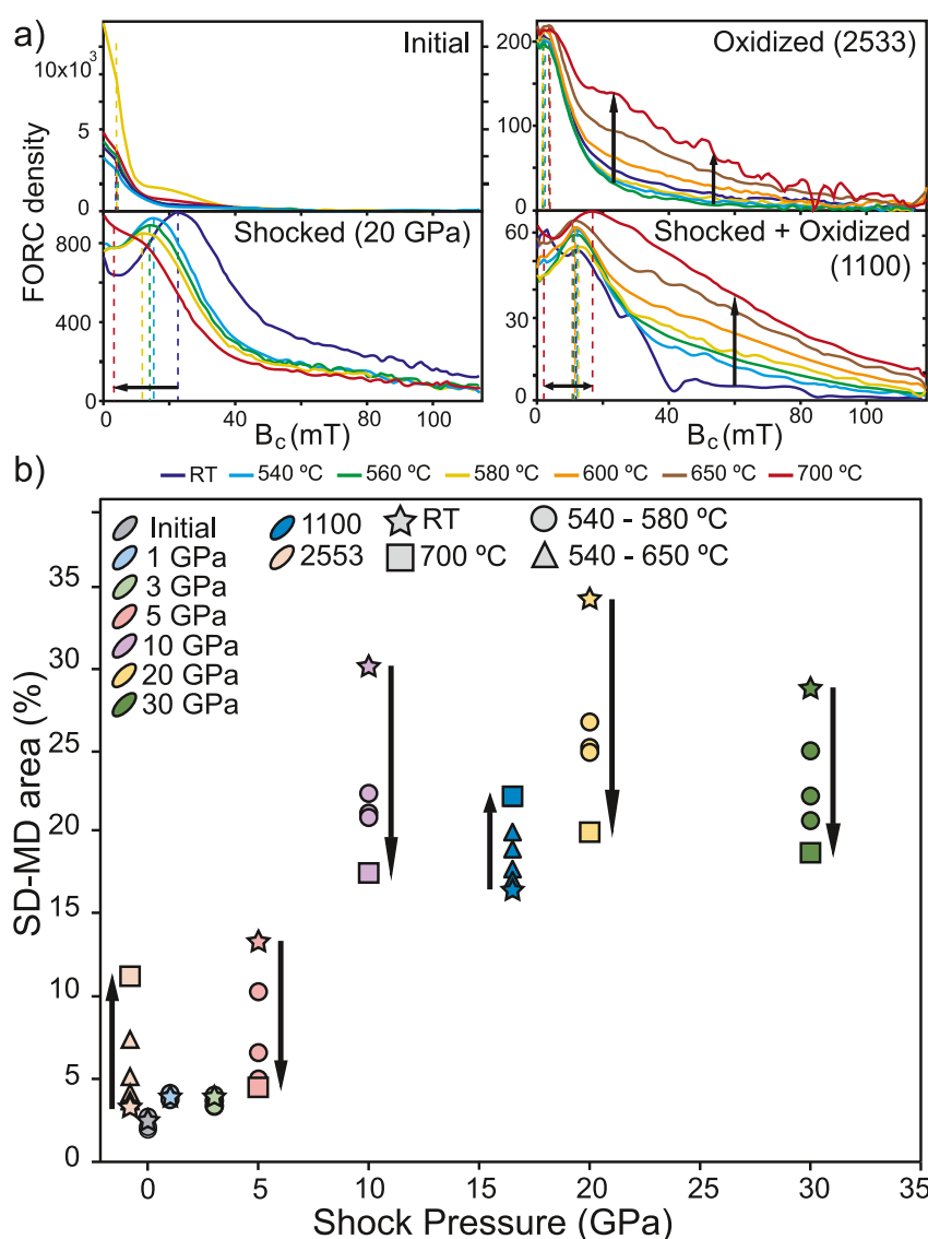
Figure 5. Evolution and variation of the FORC signal with temperature. (a) Horizontal FORC density profiles along the B_u = 0 mT axis (i.e., horizontal dashed lines in Figures 3 and 4), at different temperatures, for representative samples of no and low shocked magnetite ore (Initial) and high shocked magnetite ore (20 GPa), as well as both natural granites (2,533 from Soultz and 1,100 from Chicxulub); (b) SD-MD signal area for all investigated samples. Shock pressure of 16.5 GPa for sample 1,100 is an approximation (Feignon et al., 2020). Samples that suffered no shock are plotted for clarity at -1 (sample 2,533) and 0 (Initial magnetite ore). Data of SD-MD area calculations are provided in supplemental file 1 and supplemental file 2, respectively.
