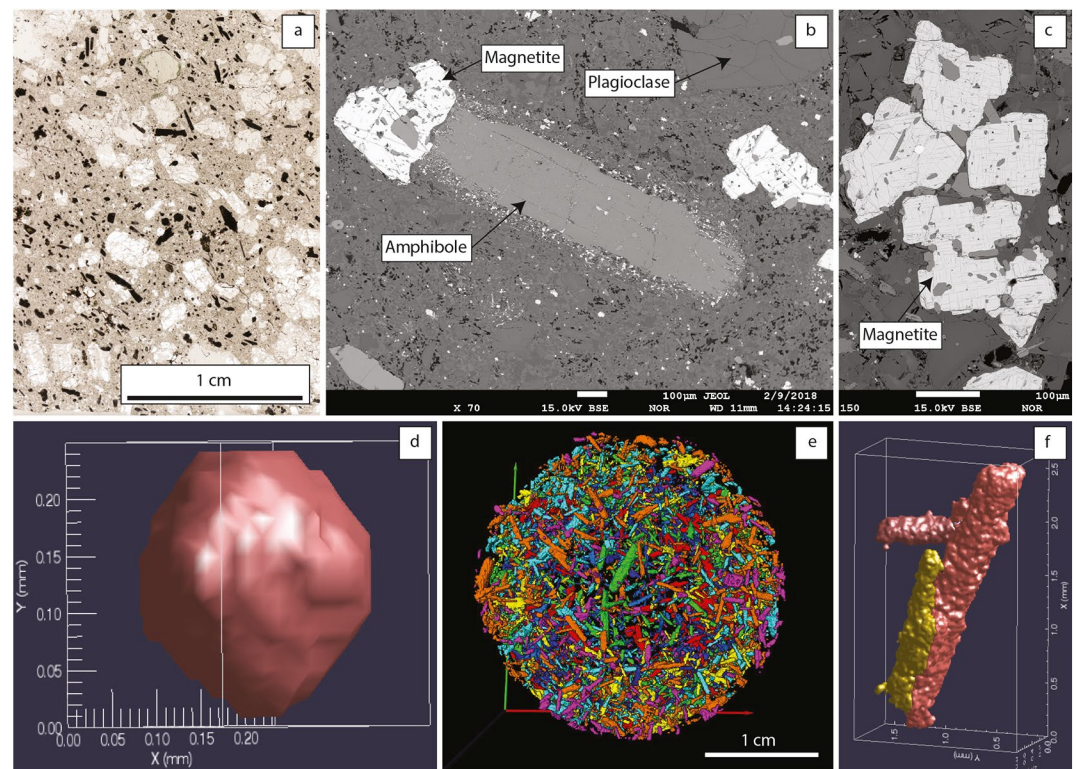
Figure 1. (a) Plane-polarized microphotograph of plagioclase- (light crystals) and amphibole- (dark and green crystals) phyric Cerro Bayo trachyandesite. (b) Back-scattered electron image of amphibole and magnetite phenocrysts in Cerro Bayo trachyandesite. Note that the breakdown rims on the amphibole consist of small magnetite and pyroxene crystals. (c) Back-scattered electron image of magnetite cluster in Cerro Bayo trachyandesite. (d) Magnetite crystal extracted with Blob3D. The magnetite crystals in Cerro Bayo generally have cubic habits. (e) Amphibole crystals extracted with Avizo from sample CB-55. The crystals are colored to distinguish different crystals. (f) Three prolate amphibole crystals from sample CB-55 separated with Blob3D.
