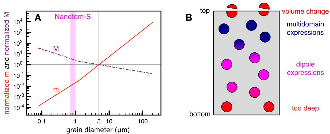
Figure 5. The spatial characterization of magnetic sources in a sample. The magnetization ( M , in purple) and magnetic moment ( m , in red) of spherical grains arising from a thermoremanent magnetic state vary as a function of their diameter (a). The data are normalized to the values for a 5\text{ }\mu\text{m} grain. The detection limit of the Nanotom-S microCT is pink. Figure adapted from Figure 7.10 in Tauxe (2010), based on data presented in Dunlop and Özdemir (1997). How well MMT can determine the magnetization of the grains (represented by the circles) depends on their depths in the sample (b). The grains at the surface are cut during sample preparation and therefore lose their natural magnetization (top grains, in red); the magnetic expression of shallow grains may represent a complex “multidomain” magnetic configuration (in blue); the magnetic expression of somewhat deeper grains represent their far-field, dipolar, magnetic moment (in pink); and the magnetic anomalies arising from grains that are too deep in the sample (in red) may be too weak to be properly inverted into the magnetization of the grains.
