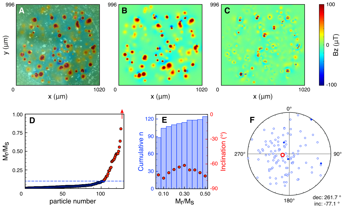
Figure 3. Results of Quantum Diamond Microscope experiments on the synthetic sample. The optical microscopy image is in the background in gray-scale (a), the map of the magnetic flux density perpendicular to the surface (in color) is super-positioned with 50% transparency. The outcome of the forward calculations is in b, the map of the residuals is in (c) The theoretical M_r/M_s ratios of the individual magnetite grains (see main text) are sorted in increasing order (d). The graph is clipped at the theoretical maximum M_r/M_s ratio of 1; one grain with a M_r/M_s ratio of 2.42 is not shown, as indicated by the red arrow. For cumulative bins of M_r/M_s ratios, the cumulative n is plotted together with the resulting inclination for the selected grains (e). For grains with M_r/M_s ratios < 0.10 (blue dashed line in d), the resulting direction is closest to the expected direction. For these grains, the distribution of their individual directions is in f (open symbols pointing upwards, closed symbols downwards), with the resulting direction in red.
