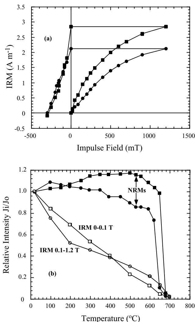
Figure 1. (a) IRM acquisition and back field demagnetization of the Suweiyi Formation red bed samples and (b) thermal demagnetization of NRM and IRMs acquired in a 1.2 T field indicate haematite is the dominant magnetic mineral.
