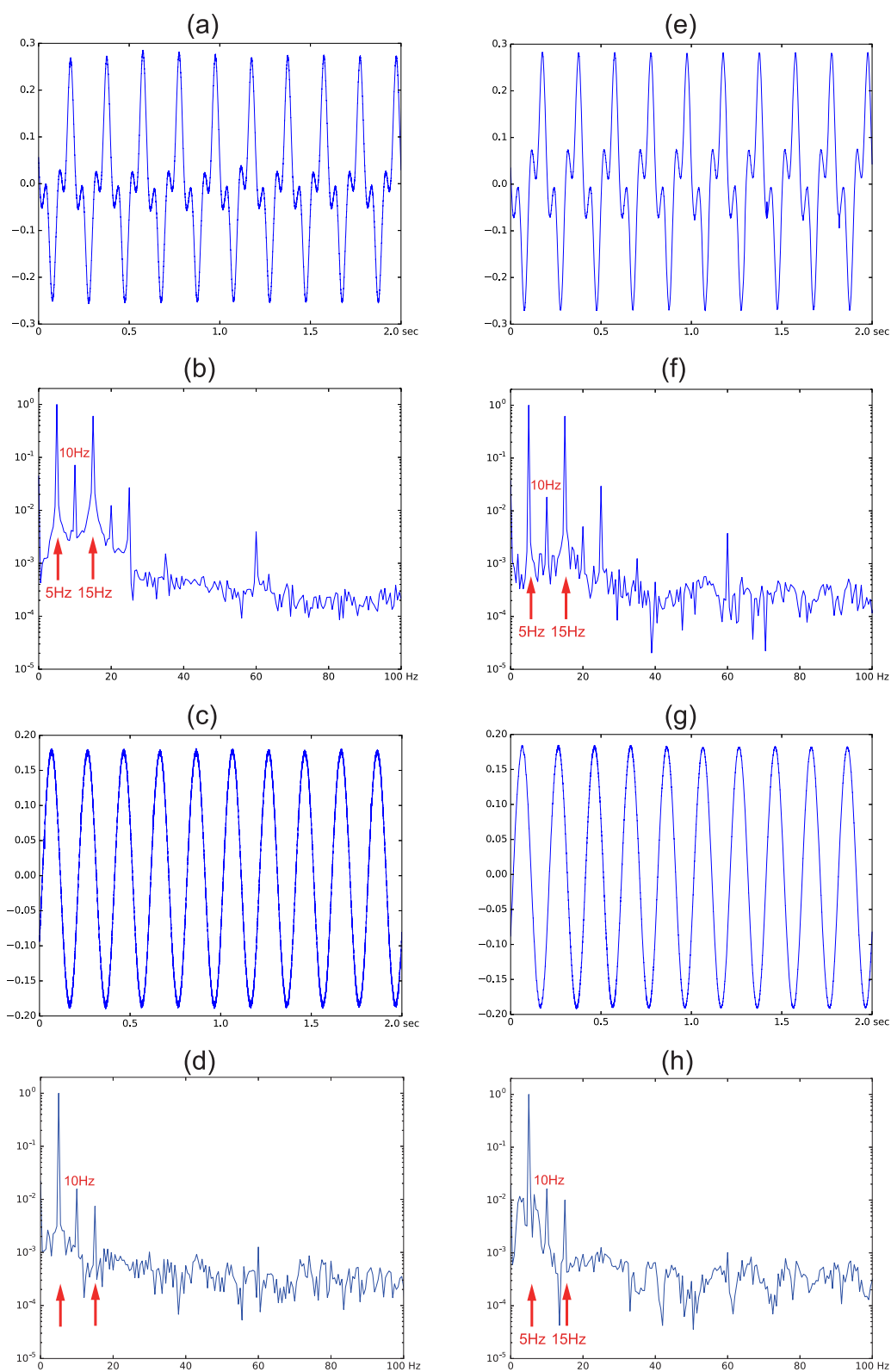
Figure 7. Waveforms and their corresponding FFT spectrum, recorded for 2 s using the test coil with the supplied current of 2 mA in two different orientations, (a–d) 30° and (e–h) 60°. The waveforms were measured in the (a, e) H mode and (c, g) F mode.
