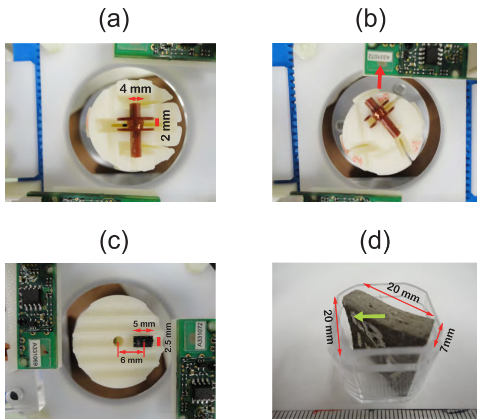
Figure 4. (a) Dipole-simulating coil ( 4 \times 2 mm) placed at the center of the sample holder. (b) The same coil with the offset of 4 mm away from the spinning axis in the orientation 30^\circ CCW with respect to the sensing direction of the MI sensor (red arrow). (c) A mini-core sample of basalt (5 mm long, 2.5 mm in diameter, weighing 87 mg), with the axial ARM of 5.3 \times 10^{-6} Am 2 , placed on a special holder for simulating a dipole with the offset of 6 mm. The amount of the offset was varied by changing the distance from the spinning axis to the middle of the mini-core. (d) A fragment of a Japanese porcelain sample ( 20 \times 20 \times 7 mm), with the ARM in the designated direction (green arrow), in a plastic 1 inch cube.
