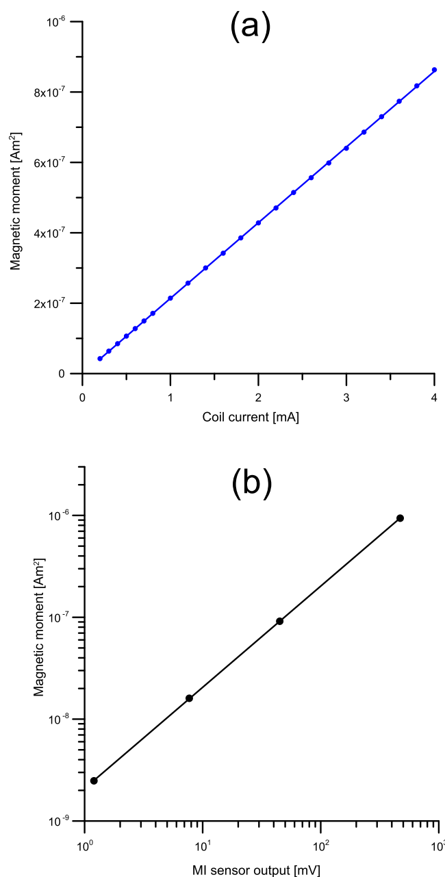
Figure 5. (a) Magnetic moment ( \text{Am}^2 ) versus supplied current (mA) at the sensor distance of 17 mm. (b) Magnetic moment ( \text{Am}^2 ) versus MI sensor output ranging in the three orders of magnitudes in mV.
