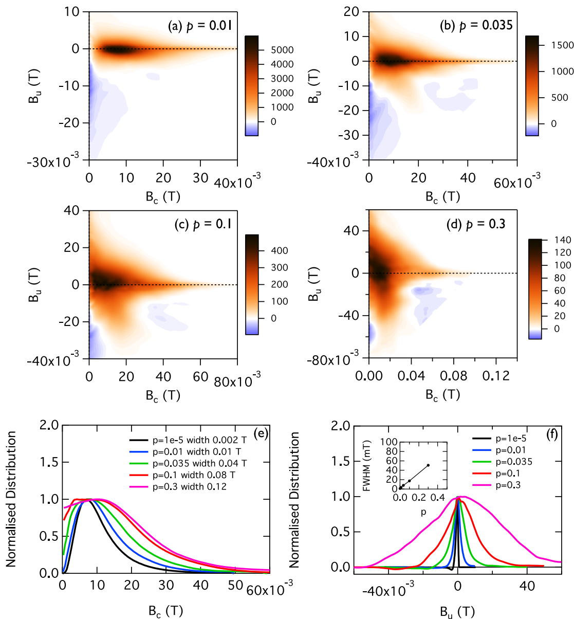
Figure 5. LLG simulations for randomly packed, randomly oriented, cubic particles with \langle 111 \rangle easy axes. (a) Simulation parameters: p = 0.01 , N = 250 , N_{avg} = 200 , N_{FORC} = 100 , B_c = 50 mT, B_u = 10 mT, \Delta B = 0.6 mT. VARIFORC smoothing parameters: \{s_{c0}, s_{c1}, s_{b0}, s_{b1}, \lambda_c, \lambda_b\} = \{3, 7, 2, 7, 0.2, 0.2\} . (b) Simulation parameters: p = 0.035 , N = 250 , N_{avg} = 200 , N_{FORC} = 100 , B_c = 60 mT, B_u = 40 mT, \Delta B = 1 mT. VARIFORC smoothing parameters: \{s_{c0}, s_{c1}, s_{b0}, s_{b1}, \lambda_c, \lambda_b\} = \{3, 7, 3, 7, 0.2, 0.2\} . (c) Simulation parameters: p = 0.1 , N = 250 , N_{avg} = 200 , N_{FORC} = 100 , B_c = 100 mT, B_u = 50 mT, \Delta B = 1.5 mT. VARIFORC smoothing parameters: \{s_{c0}, s_{c1}, s_{b0}, s_{b1}, \lambda_c, \lambda_b\} = \{3, 7, 3, 7, 0.2, 0.2\} . (d) Simulation parameters: p = 0.3 , N = 250 , N_{avg} = 200 , N_{FORC} = 100 , B_c = 100 mT, B_u = 60 mT, \Delta B = 1.6 mT. VARIFORC smoothing parameters: \{s_{c0}, s_{c1}, s_{b0}, s_{b1}, \lambda_c, \lambda_b\} = \{9, 9, 9, 9, 0.2, 0.2\} . (e) Horizontal profiles at B_u = 0 . The profiles were obtained by summing the FORC distribution inside a window of specified width, centered on the B_u = 0 axis, and normalizing to the peak value. (f) Vertical profiles at B_c = 7 mT. Inset shows the FWHM of the vertical profile as a function of packing fraction ( p ).
