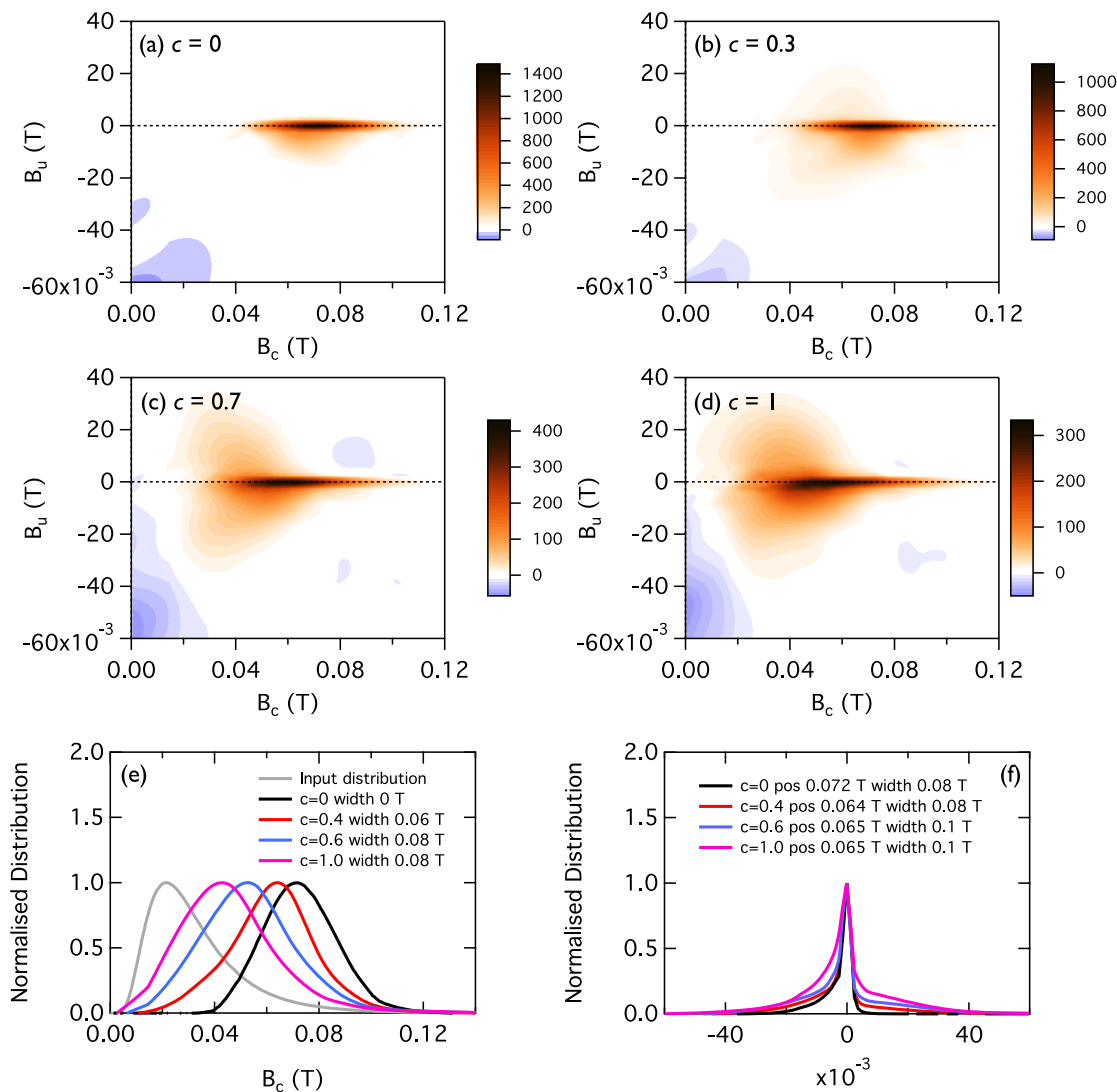
Figure 7. LLG simulations for the chain configurations shown in Figure 6. (a) Simulation parameters: c = 0 , N_{avg} = 25 , N_{FORC} = 100 , B_c = 160 mT, B_u = 60 mT, \Delta B = 2.5 mT. VARIFORC smoothing parameters: \{s_{c0}, s_{c1}, s_{b0}, s_{b1}, \lambda_c, \lambda_b\} = \{12, 12, 2, 12, 0, 0\} . (b) Simulation parameters: c = 0.3 , N_{avg} = 25 , N_{FORC} = 100 , B_c = 160 mT, B_u = 60 mT, \Delta B = 2.5 mT. VARIFORC smoothing parameters: \{s_{c0}, s_{c1}, s_{b0}, s_{b1}, \lambda_c, \lambda_b\} = \{12, 12, 2, 12, 0, 0\} . (c) Simulation parameters: c = 0.7 , N_{avg} = 25 , N_{FORC} = 100 , B_c = 160 mT, B_u = 60 mT, \Delta B = 2.5 mT. VARIFORC smoothing parameters: \{s_{c0}, s_{c1}, s_{b0}, s_{b1}, \lambda_c, \lambda_b\} = \{12, 12, 2, 12, 0, 0\} . (d) Simulation parameters: c = 1 , N_{avg} = 25 , N_{FORC} = 100 , B_c = 160 mT, B_u = 60 mT, \Delta B = 2.5 mT. VARIFORC smoothing parameters: \{s_{c0}, s_{c1}, s_{b0}, s_{b1}, \lambda_c, \lambda_b\} = \{12, 12, 2, 12, 0, 0\} . (e) Horizontal profiles at B_u = 0 . The profiles were obtained by summing the FORC distribution inside a window of specified width, centered on the B_u = 0 axis, and normalizing to the peak value. (f) Vertical profiles taken at the indicated position (corresponding to the peak position of the corresponding horizontal profile) and summed over a window with the specified width.
