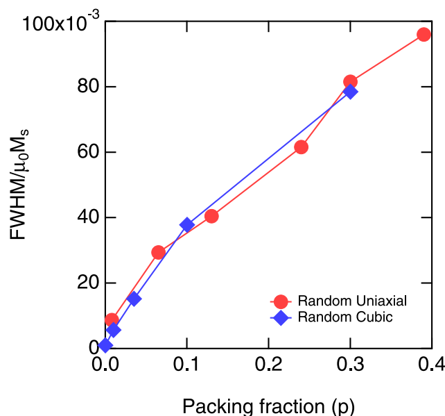
Figure 9. Scaled FWHM, i.e., FWHM (in T) divided by \mu_0 M_s for magnetite (0.603 T), extracted from low-coercivity vertical profiles for randomly packed uniaxial (circles) and cubic (diamonds) particles as a function of packing fraction ( p ). Profiles were taken at coercivities of 10 and 7 mT for uniaxial and cubic particles, respectively. FWHM was defined in this case as twice the half width to half maximum extracted from the upper half (i.e., B_u > 0 ) of the vertical profile.
